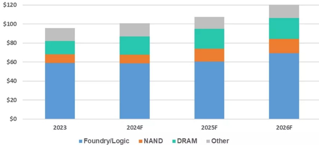
SEMI 2024 Year-end Wafer Fab Equipment Forecast by Application (US$ Billion)
